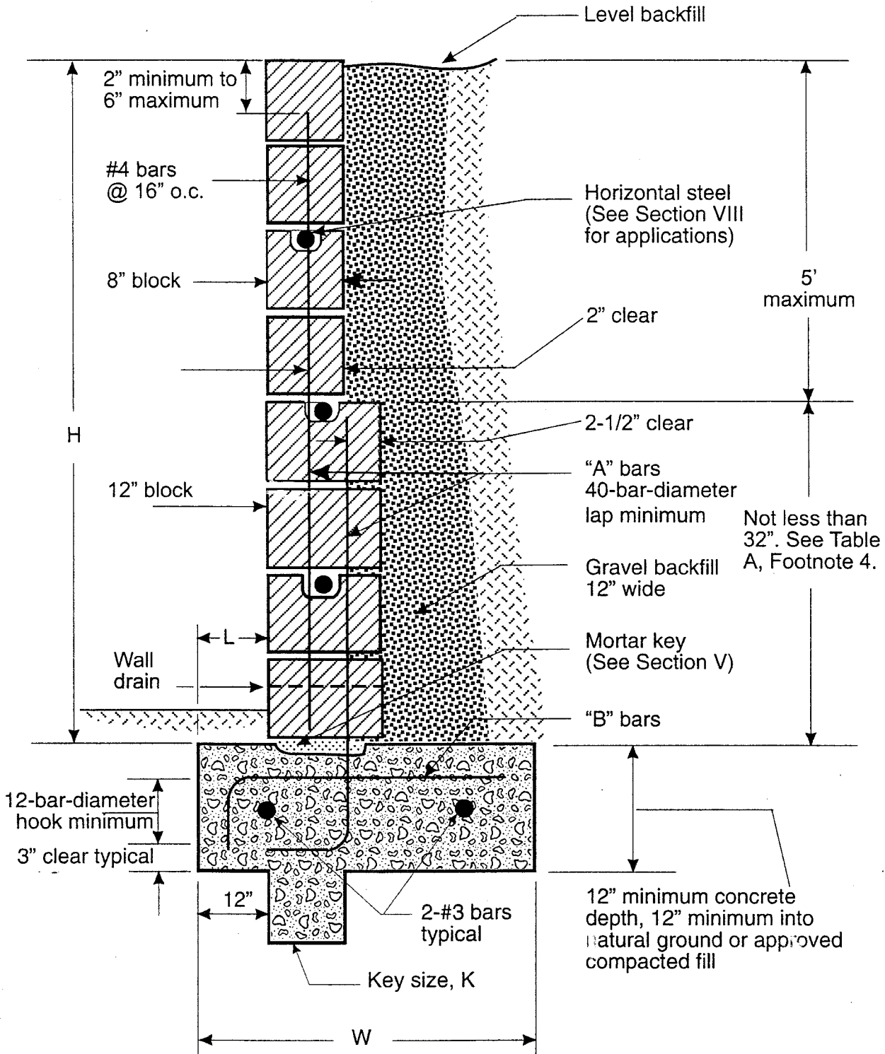
Figure 2/Type V retaining wall with level backfill
